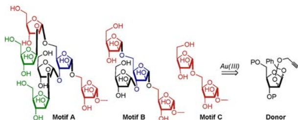
Figure 1. Mtb cell wall motifs A–C and the strategy.
