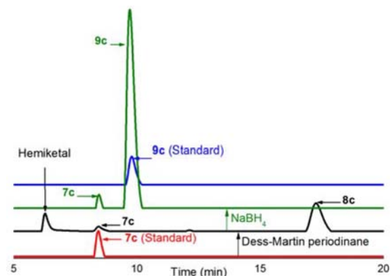
Figure 2. Representative UPLC trace for the conversion of \beta -Ribf substrate 7c to \beta -Araf product 9c .
