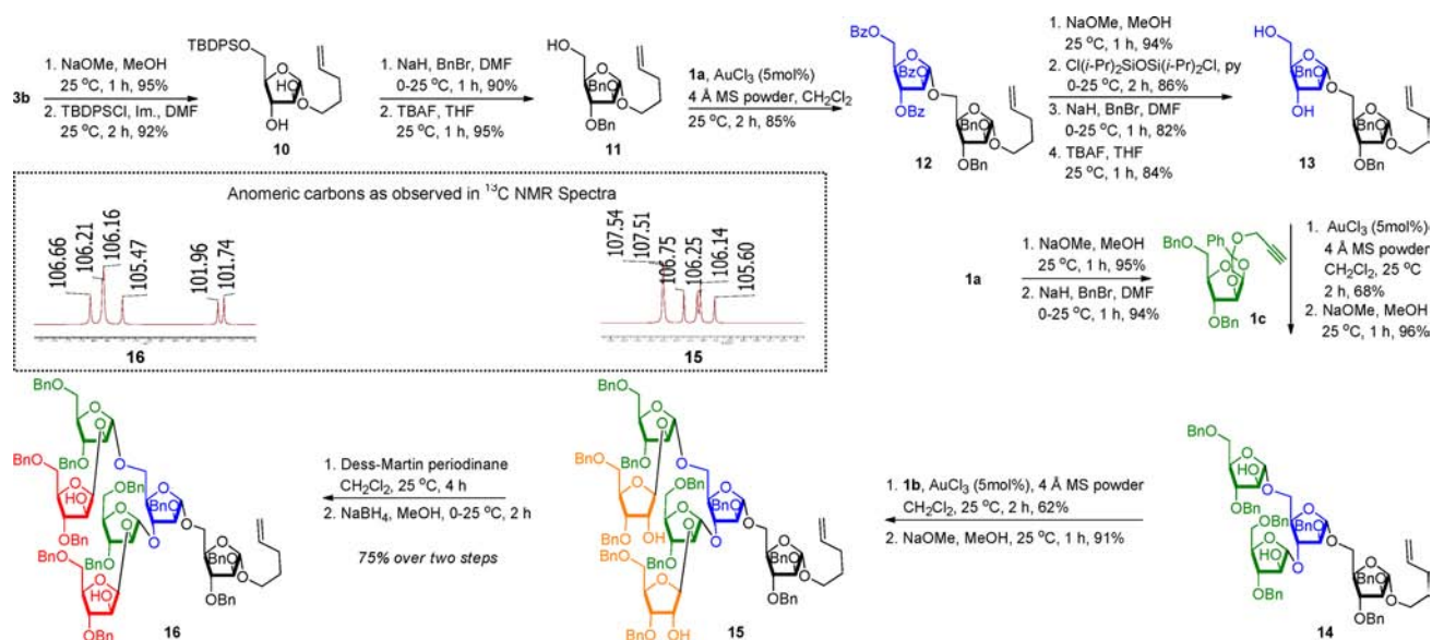
Scheme 3. Synthesis of Arabinan Motifs of M. tuberculosis
