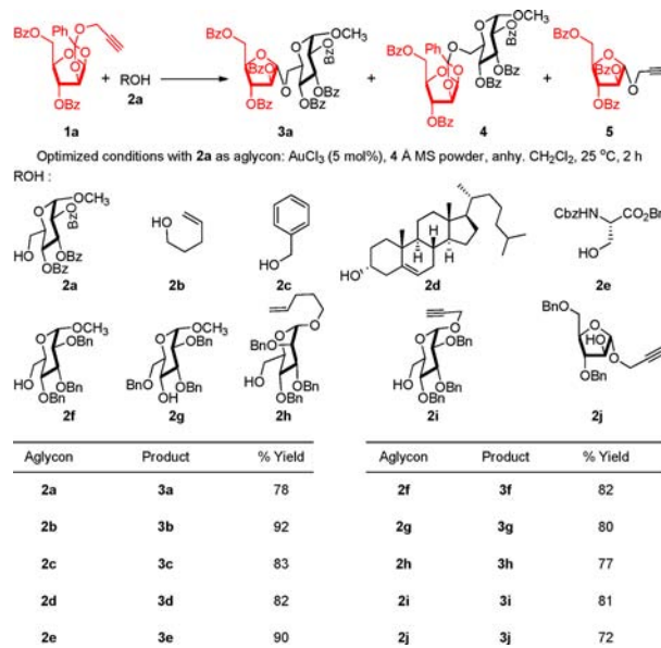
Scheme 1. Propargyl 1,2-Orthoesters for α-Arabinofuranosides
